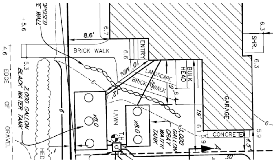
Figure 1. Blackwater Storage Tank Configuration
